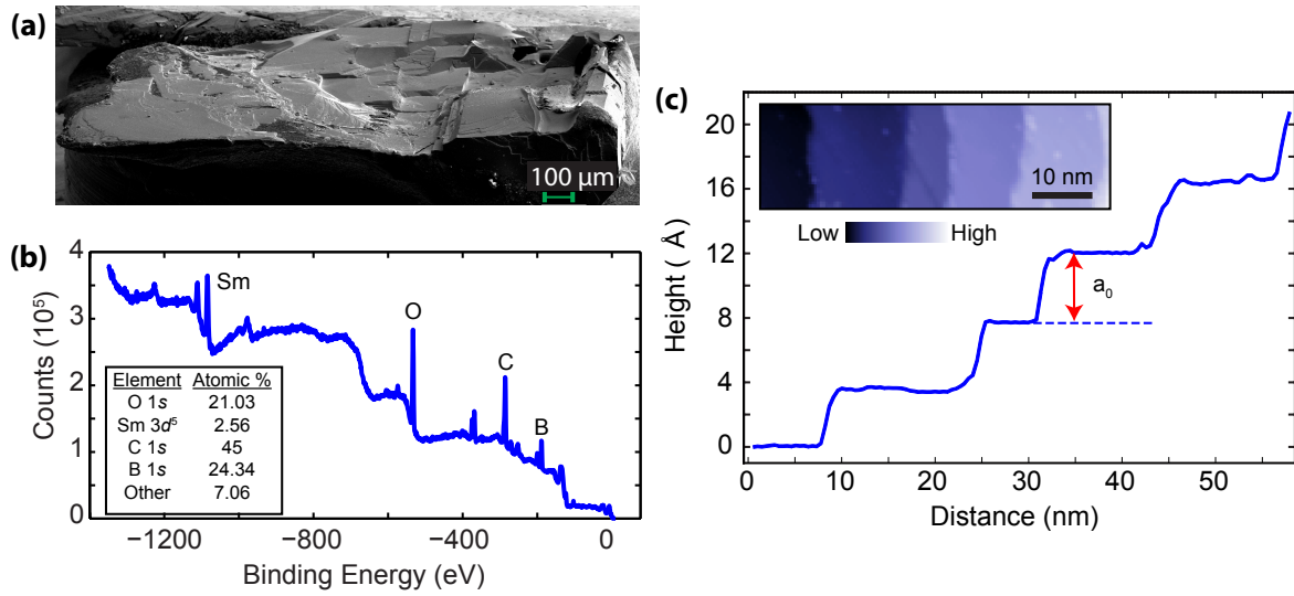
Figure 3.3: Surface characterization of \text{SmB}_6 . (a) Scanning electron microscope (SEM) image of one of the \text{SmB}_6 crystals studied. All four nanoscale morphologies were observed on this cleaved surface. (b) X-ray photoemission spectroscopy (XPS) spectrum of the surface shown in (a). Annotated peaks correspond to the binding energies of the respective atoms. Inset: Atomic composition extracted from the XPS spectrum. The surface ratio of Sm:B is 1:9.5. (c) Topographic linecut across five atomically flat terraces. The difference in the vertical height between adjacent terraces is a_0 . Inset shows a 50 \text{ nm} \times 15 \text{ nm} topography of these terraces. ( T = 7 \text{ K} ; setpoint voltage V_s = -100 \text{ mV} ; junction resistance R_J = 10 \text{ G}\Omega .) (a) and (b) were acquired after STM experiments were completed and the crystal was removed from the cryostat.
