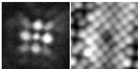
Fig. 2. Simultaneously obtained (a) LDOS map and (b) topography of a 32 Å square region, centered on a single vacancy resonance.
